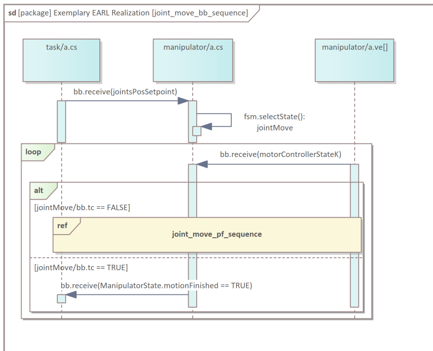
Figure 25: jointMove/bb – main sequence of actions execution
