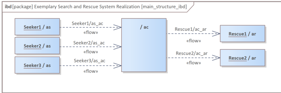
Figure 30: The structure of an exemplary instance of Search and Rescue System
