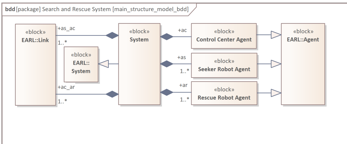
Figure 28: The composition of Search and Rescue System
