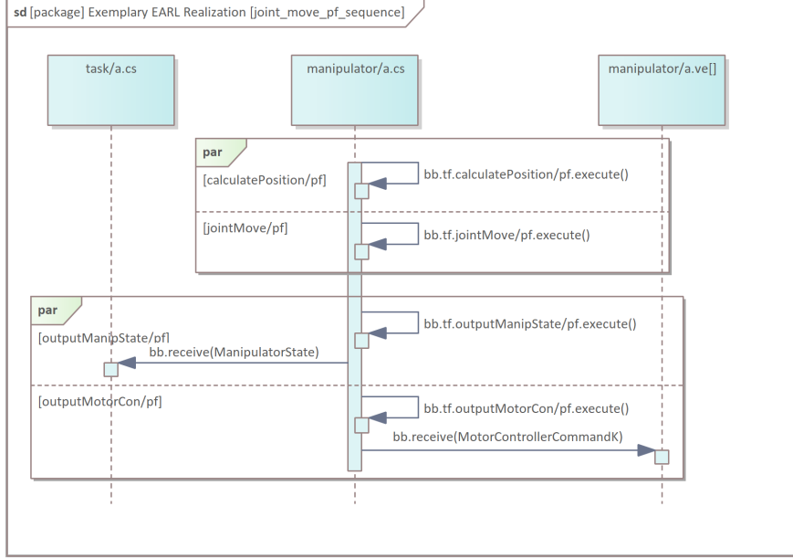
Figure 26: jointMove/bb – main sequence of associated pf execution
