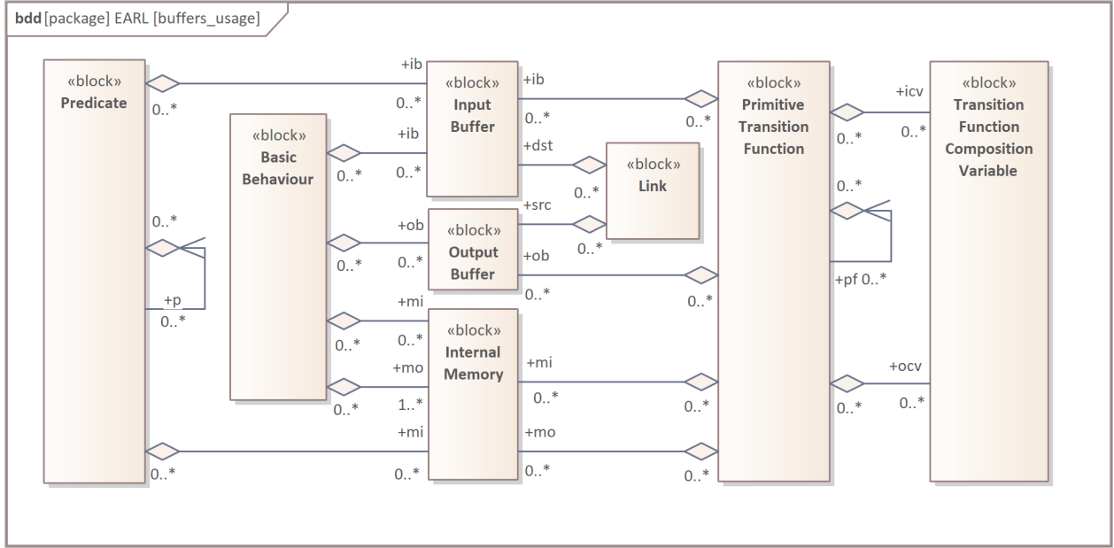
Figure 11: The utilisation of Buffers, Transition Function Composition Variables and Internal Memory by: Primitive Transition Function, Predicate and Links
