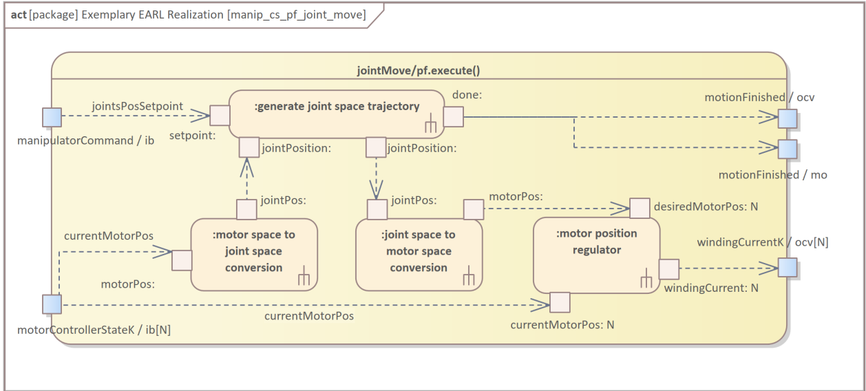
Figure 23: manip/a.cs.jointMove/pf.execute() – operation definition
