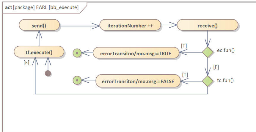
Figure 10: Basic Behaviour.execute() operation
