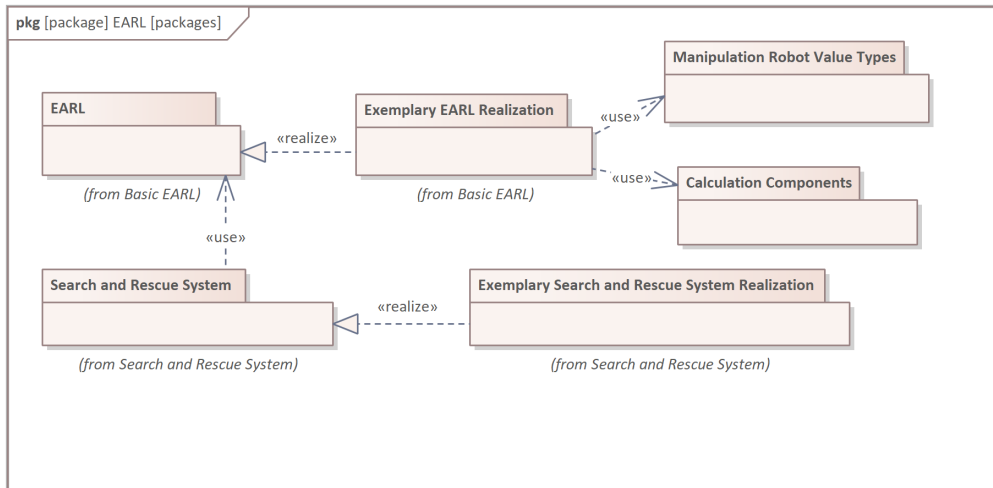
Figure 1: EARL packages dependencies
