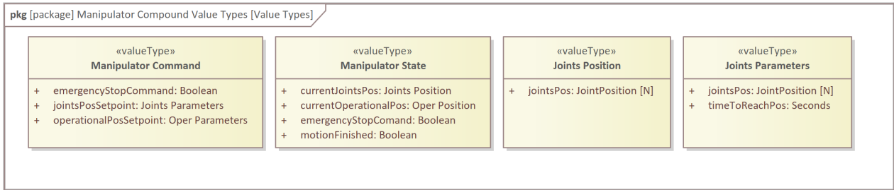
Figure 19: valueTypeS transmitted within the system
