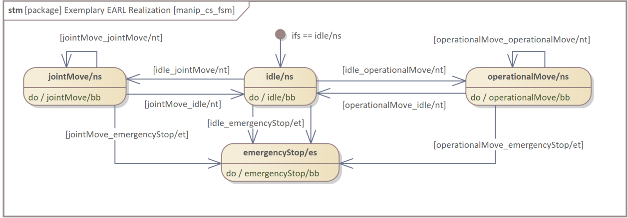
Figure 22: manip/a.cs.fsm definition. Conditions of transitions between FSM States are specified in Table 4
